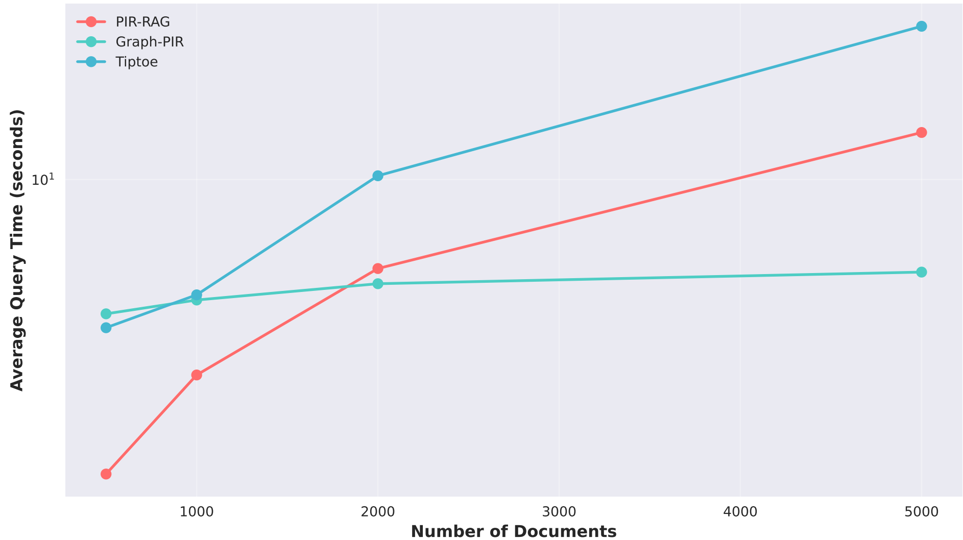
Query Time Scalability
