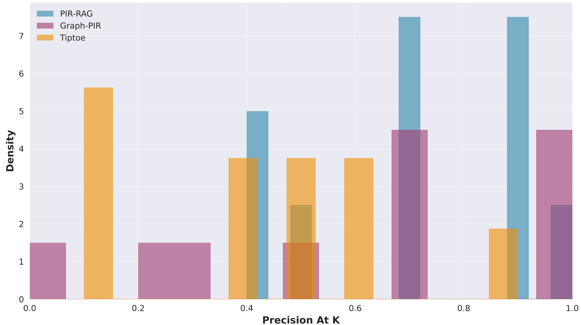
Precision@K Distribution
