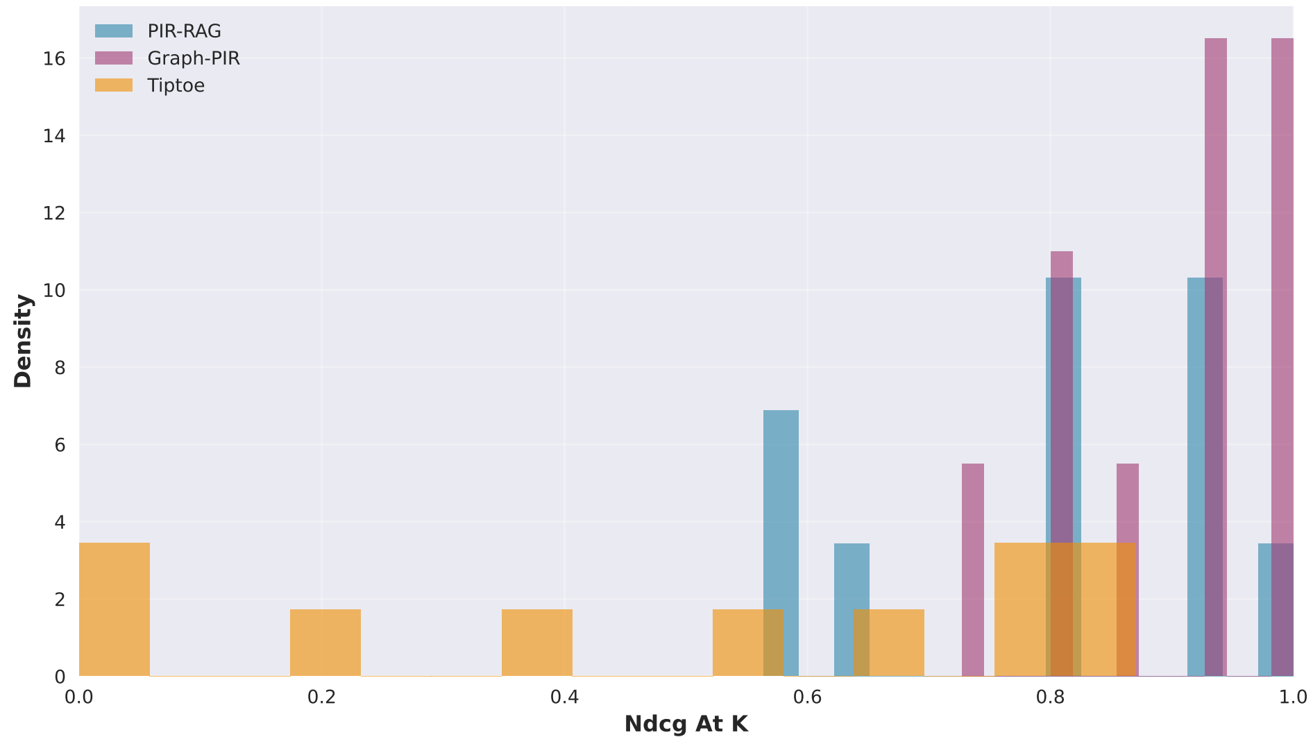
NDCG@K Distribution
