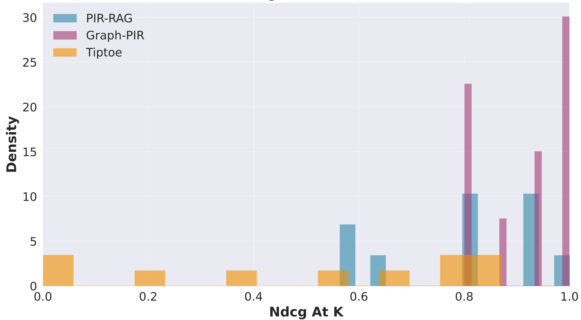
NDCG@K Distribution
