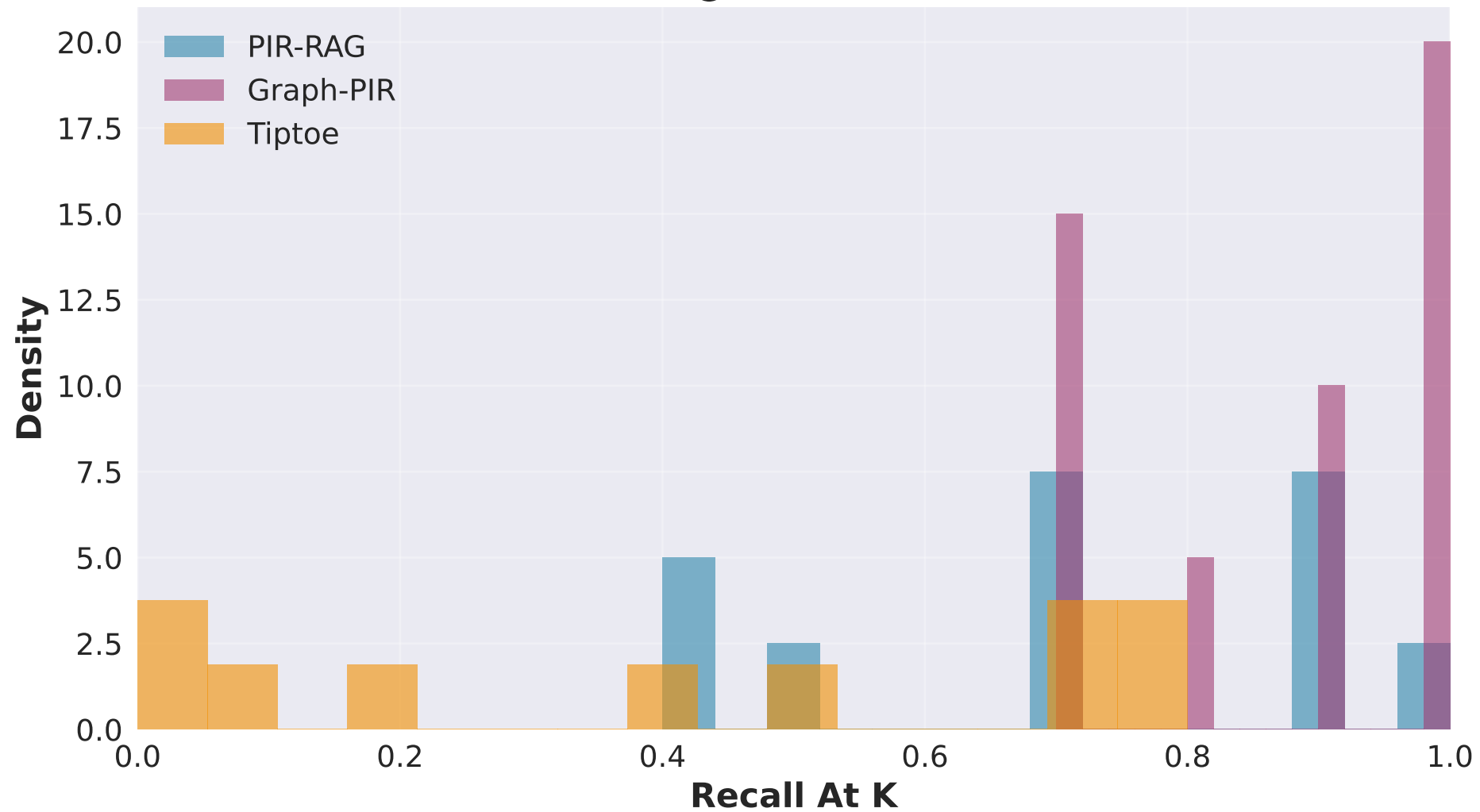
Recall@K Distribution
