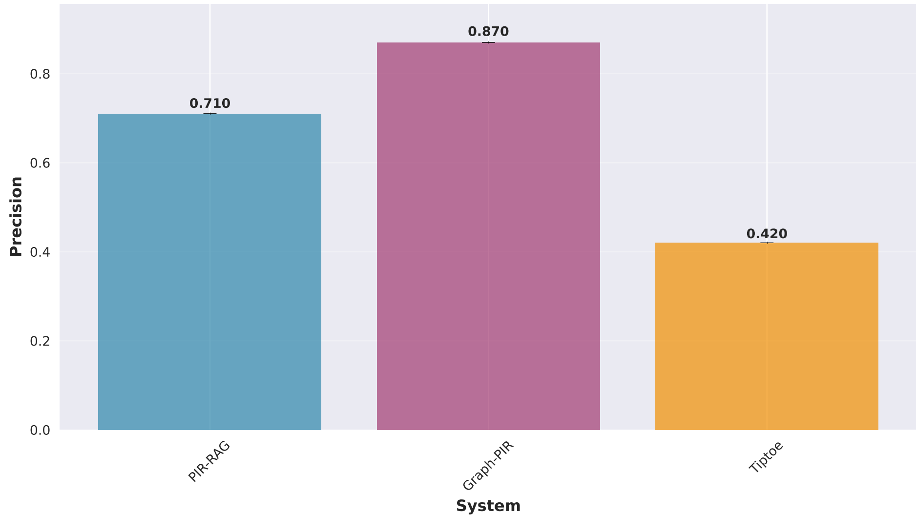
Precision@K Performance Comparison
