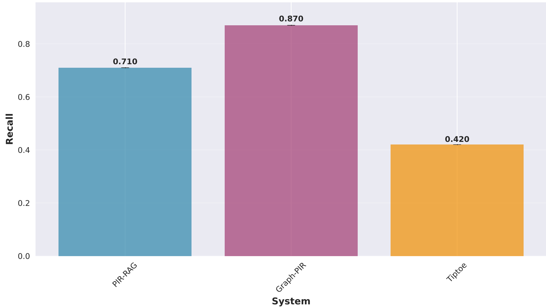
Recall@K Performance Comparison
