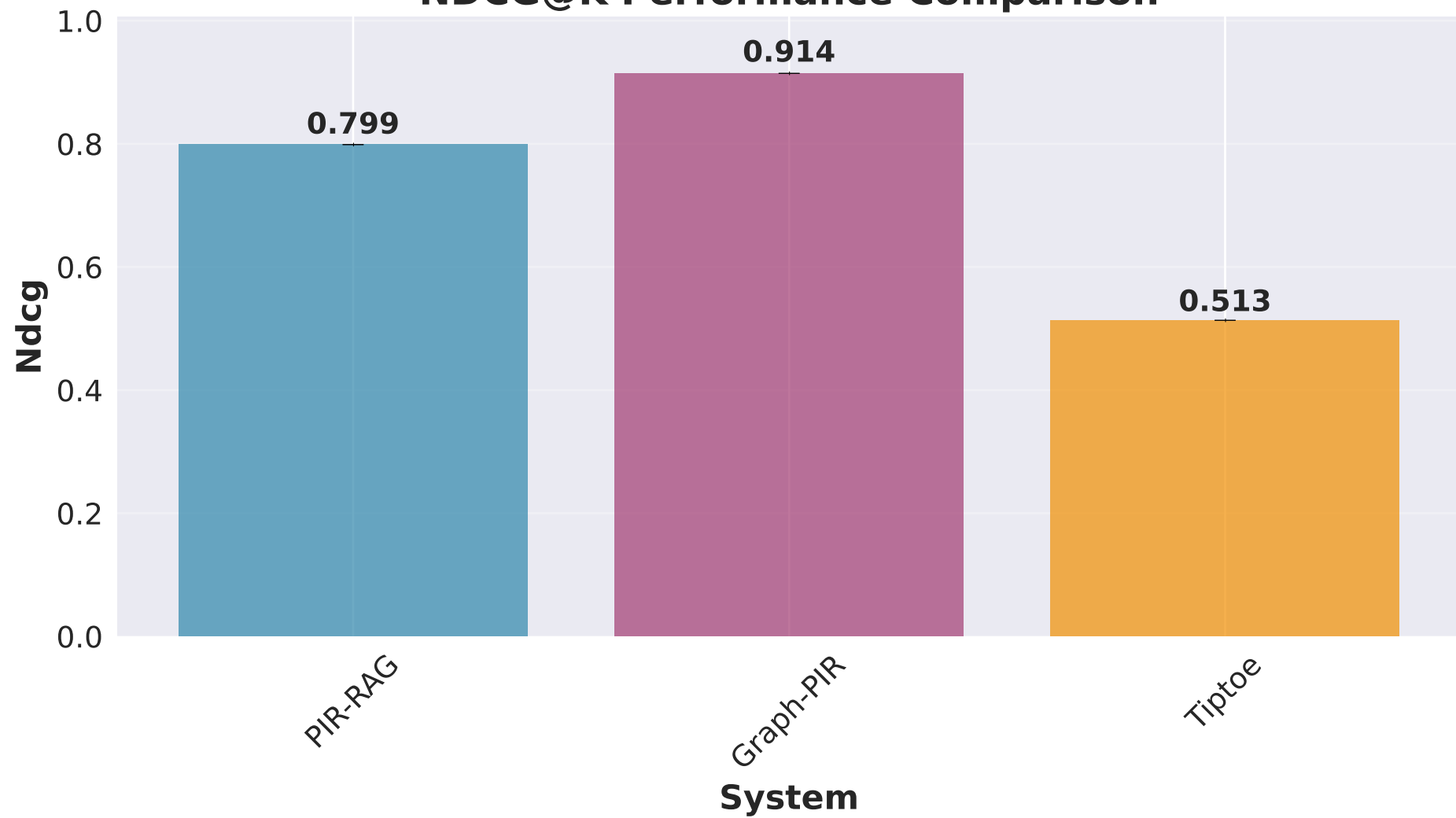
NDCG@K Performance Comparison
