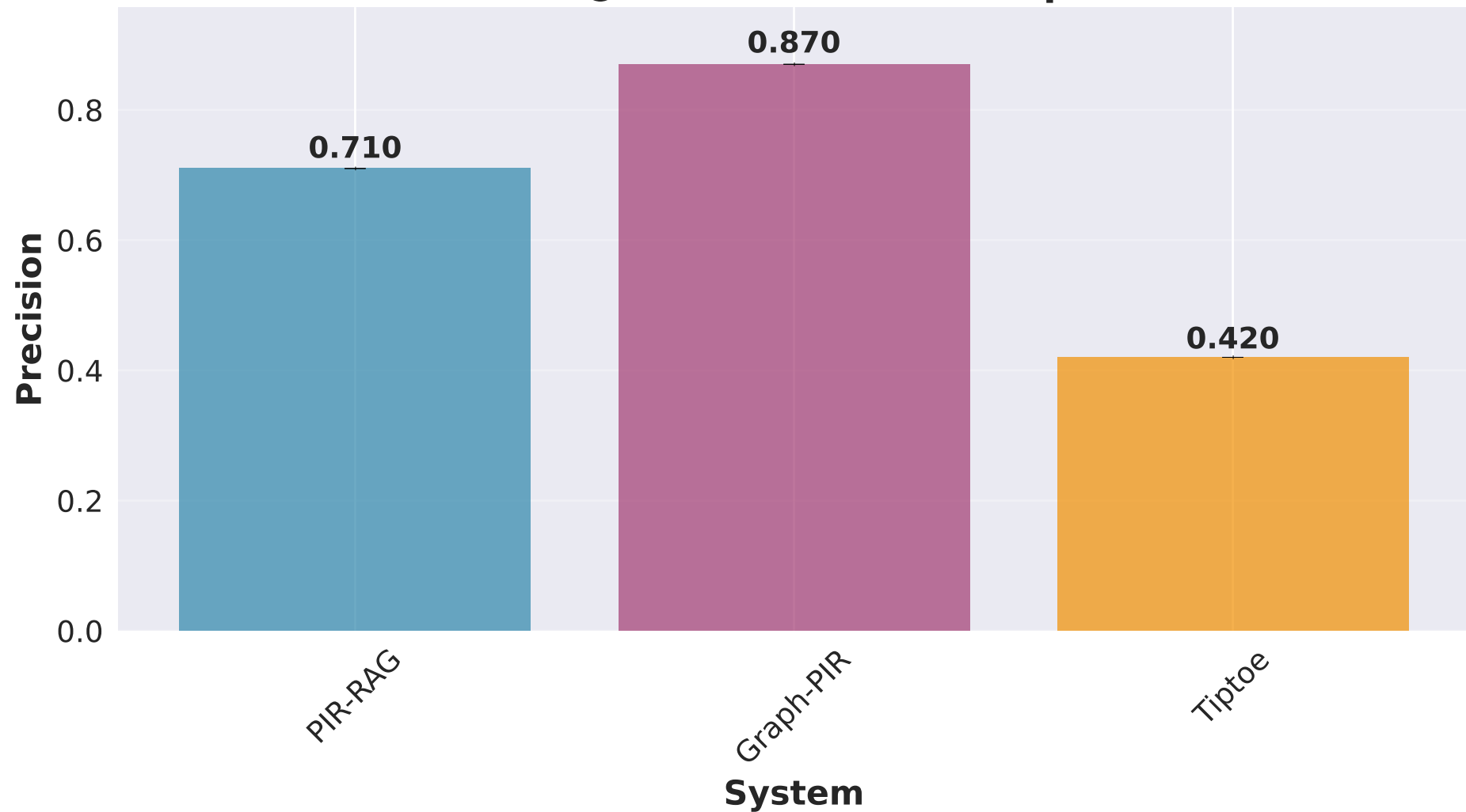
Precision@K Performance Comparison
