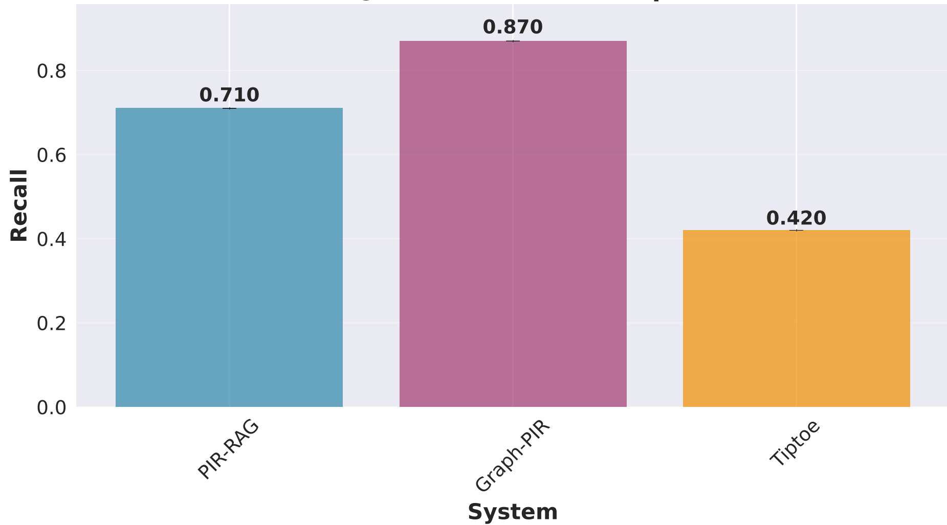
Recall@K Performance Comparison
