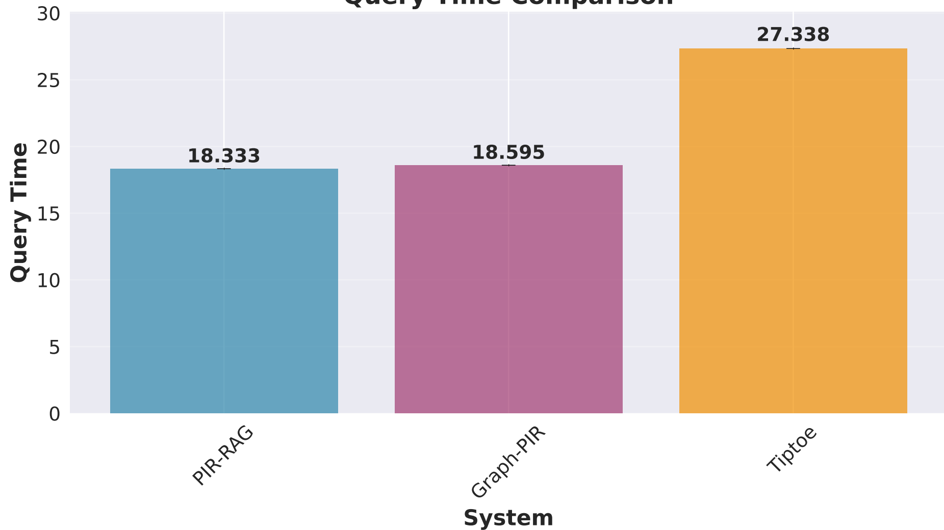
Query Time Comparison
