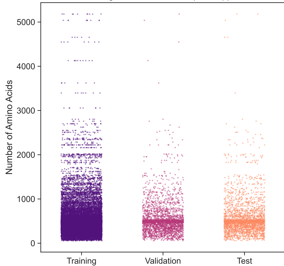
Target Size Distribution (biosnap)
