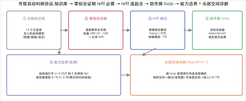
Fig. 1 — Protocol overview. The four-stage trustworthy autoresearch protocol instantiated on real DJI M100 UAV energy modeling and energy-aware path planning, with measured numbers per stage: (i) a knowledge base of 14 published models; (ii) a zero-fit transfer benchmark showing all as-published models fail on the target platform (energy ARE 53-76%), motivating refit; (iii) a refit leaderboard selecting Tseng's polynomial (1.90%) as the loop's start; (iv) the cheat-proof loop; plus the quantified capability boundaries (energy tie, planning win) and the pre-loop headroom diagnostic. (pub/协议总览_Fig1.png)
