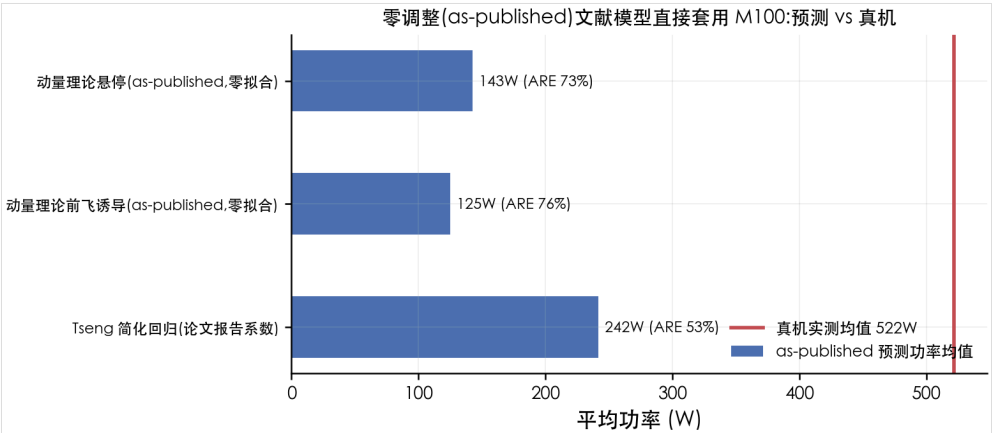
Fig. 3 — Zero-fit vs. refit. As-published (zero-fit) models fail on the target platform (energy ARE 53-76%, predicted power far below measured 522 W), while the same forms after refit reach ~2% -- the measured justification for an explicit refit stage. (pub/as_published_vs_refit.png)
