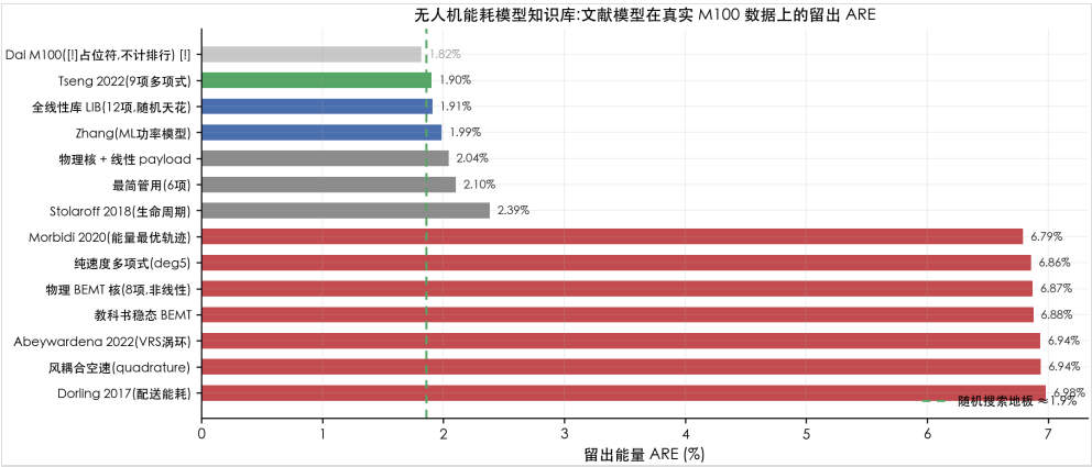
Fig. 2 — Knowledge-base leaderboard. All 14 literature UAV energy models, refit on the frozen M100 evaluator (energy ARE, lower is better). Data-driven models (Tseng 1.90%, linear LIB 1.91%) dominate; all physics forms stay 6.7-7.0% even after refit. (pub/模型知识库排行榜.png)
