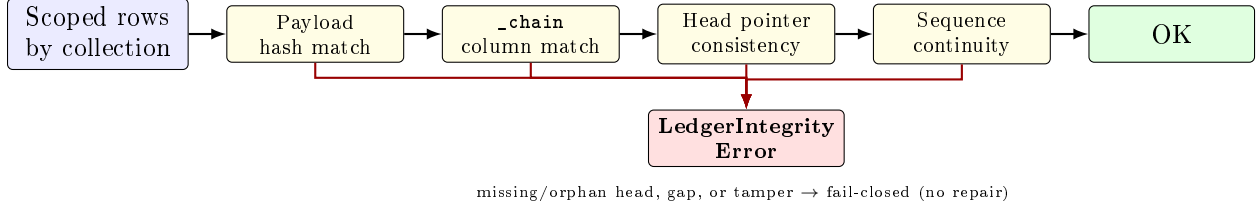
Figure 5: verify_scoped_chain recomputes hashes and chain metadata, checks head pointers and sequence continuity, and raises LedgerIntegrityError on any inconsistency.
