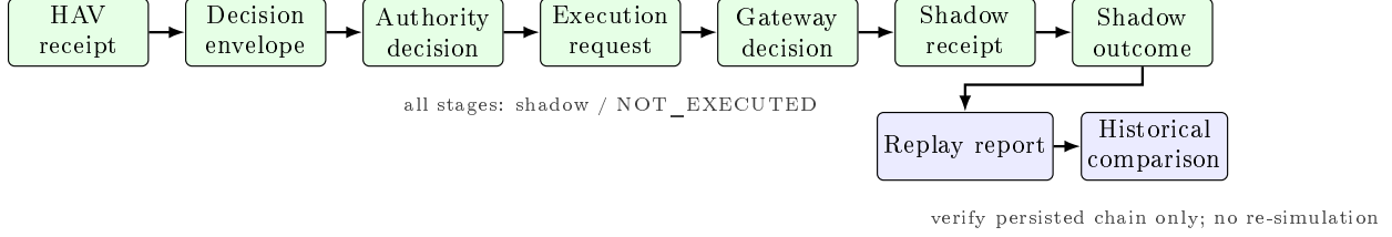
Figure 8: GRDI 0.4.0 shadow decision chain. Each box is an append-only, scope-tagged ledger collection linked through the transactional store. Replay audit reads and verifies history without invoking connectors or re-running simulation.
