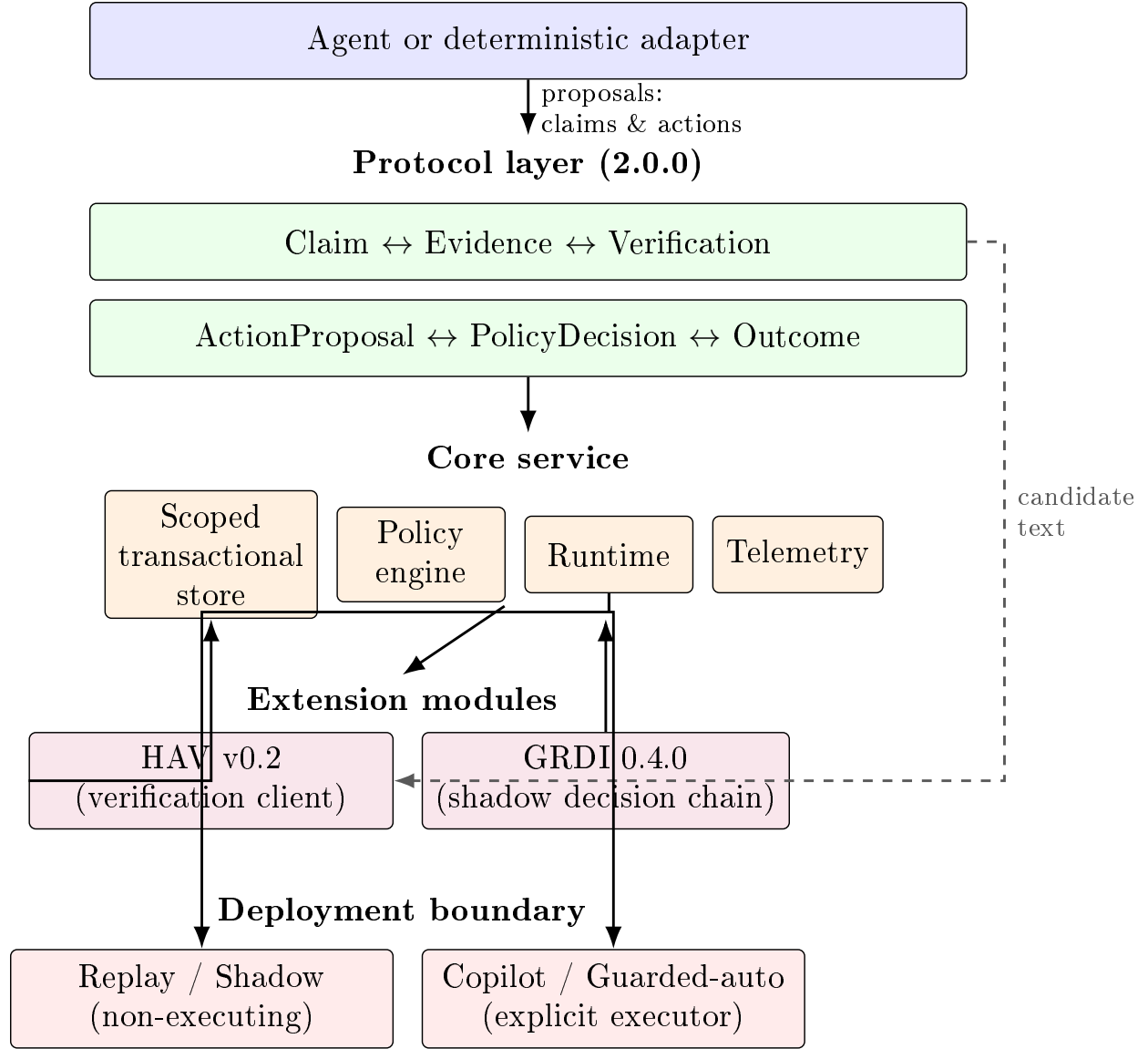
Figure 1: PhiGraph separates agent proposals from verification, policy evaluation, and execution. Core 4.1 persists scope-tagged records through a transactional store; HAV verifies candidate text against supplied state; GRDI appends a shadow decision chain through the same store. Arrows indicate recorded processing relationships, not automatic trust propagation.
