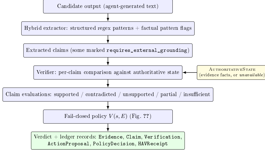
Figure 6: HAV v0.2 verification pipeline. The authoritative state is supplied by the caller, not retrieved by HAV, and merges into the verifier stage; an unavailable state is itself a valid input that the fail-closed policy (Figure ??) maps to a blocking verdict.
