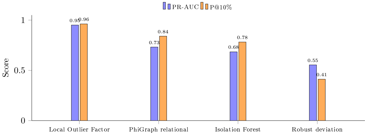
Figure 9: PR-AUC and precision at a 10% alert budget for each method on the CIC-IDS2017 Friday DDoS experiment (same run as Table ??). Local Outlier Factor dominates on both metrics; the PhiGraph relational score ranks second, ahead of Isolation Forest and robust deviation.
