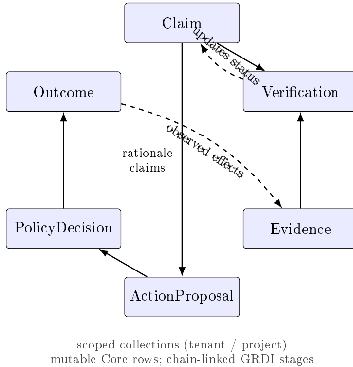
Figure 2: The protocol’s recorded lifecycle. Solid arrows show synchronous references (a verification cites claims and evidence; an action proposal cites rationale claims; a policy decision governs a proposal; an outcome follows a decision). Dashed arrows show asynchronous feedback: a verification updates claim status, and an outcome’s observed effects may be registered as new evidence for future claims. Under Core 4.1, each record type is persisted in a scope-tagged collection. The cycle is auditable, not automatic – each edge corresponds to an explicit recorded reference, not an implicit trust relationship.
