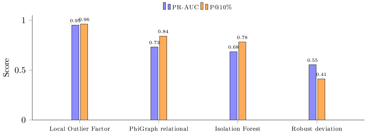
Figure 9: PR-AUC and precision at a 10% alert budget for each method on the CIC-IDS2017 Friday DDoS experiment (same run as Table 2). Local Outlier Factor dominates on both metrics; the PhiGraph relational score ranks second, ahead of Isolation Forest and robust deviation.
