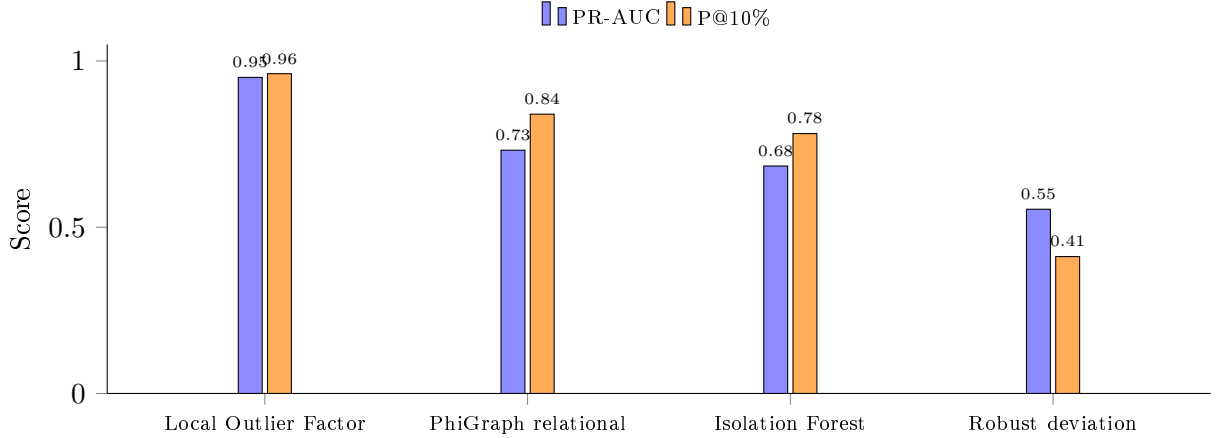
Figure 8: PR-AUC and precision at a 10% alert budget for each method on the CIC-IDS2017 Friday DDoS experiment (same run as Table 2). Local Outlier Factor dominates on both metrics; the PhiGraph relational score ranks second, ahead of Isolation Forest and robust deviation.
