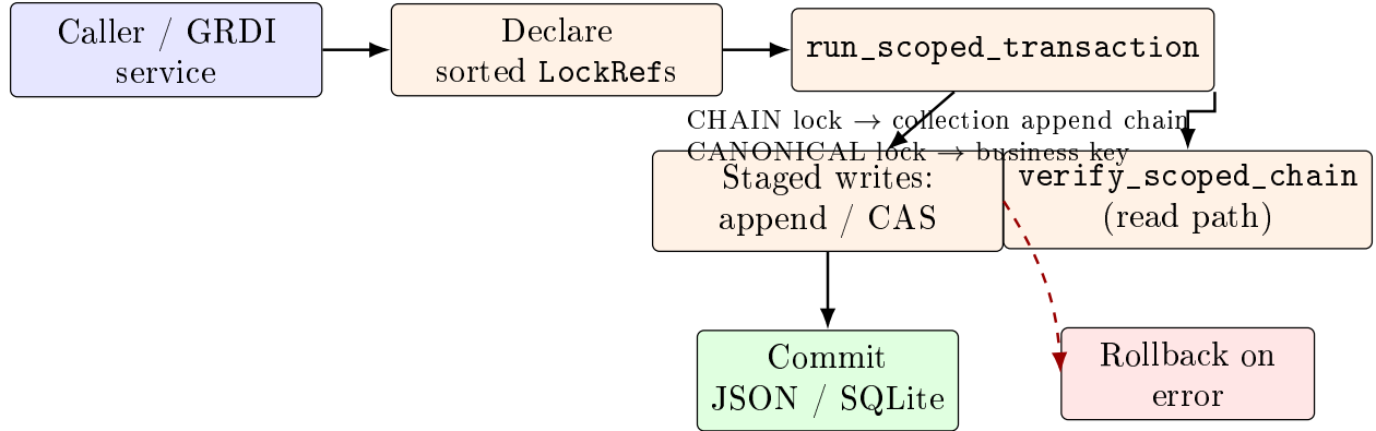
Figure 3: Scoped transactional writes require pre-declared locks and commit atomically on JSON (single-process) or SQLite ( BEGIN IMMEDIATE ). Integrity verification is a separate fail-closed read path.
