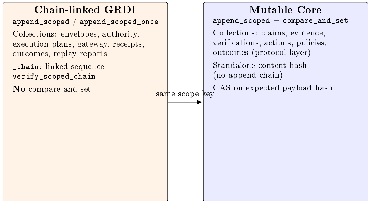
Figure 4: Chain-linked GRDI collections extend an append-only scoped hash chain; mutable Core collections support conditional updates without chain linking.
