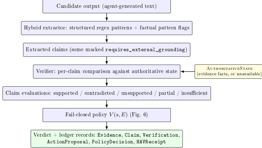
Figure 5: HAV v0.2 verification pipeline. The authoritative state is supplied by the caller, not retrieved by HAV, and merges into the verifier stage; an unavailable state is itself a valid input that the fail-closed policy (Figure 6) maps to a blocking verdict.
