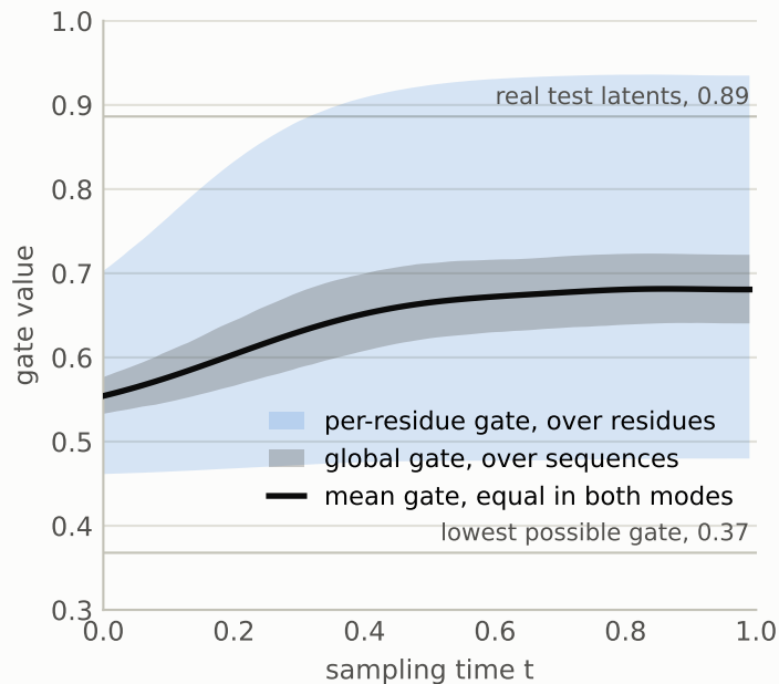
The gate over the trajectory
