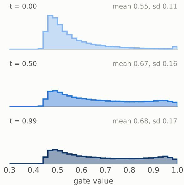
Gate values of all residues
