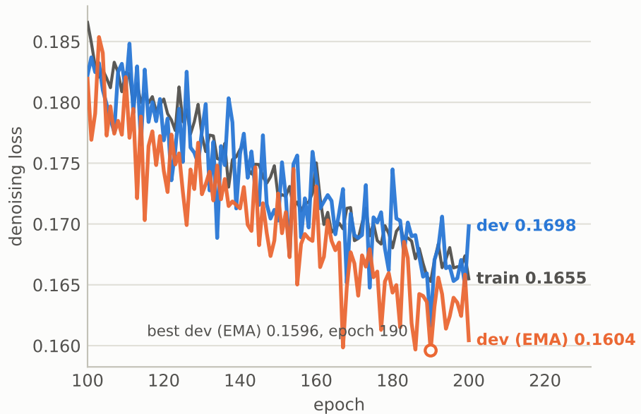
Train and dev sit on top of each other: no overfitting
