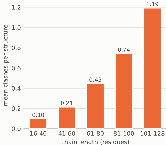
Clashes accumulate (AlphaFold: 0 at every length)
