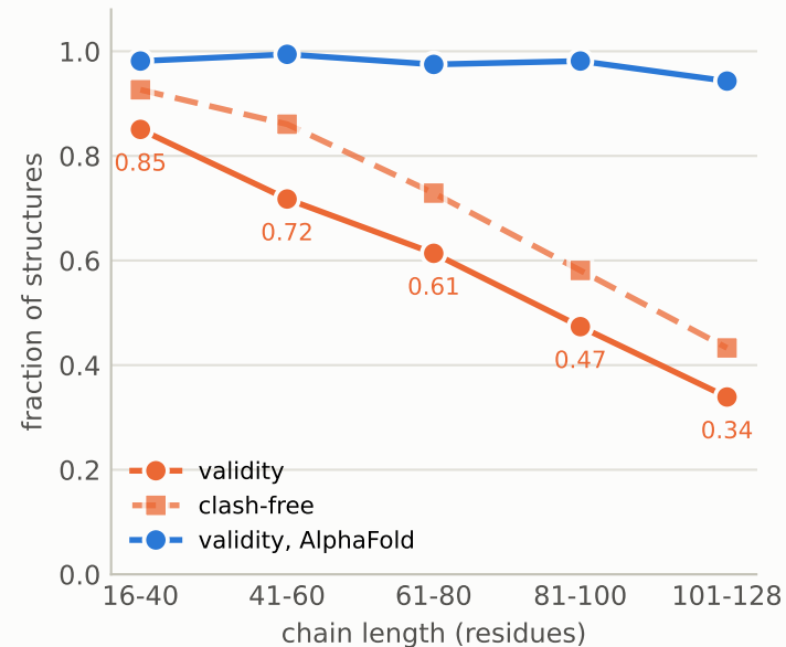
Validity falls 2.5x with length
