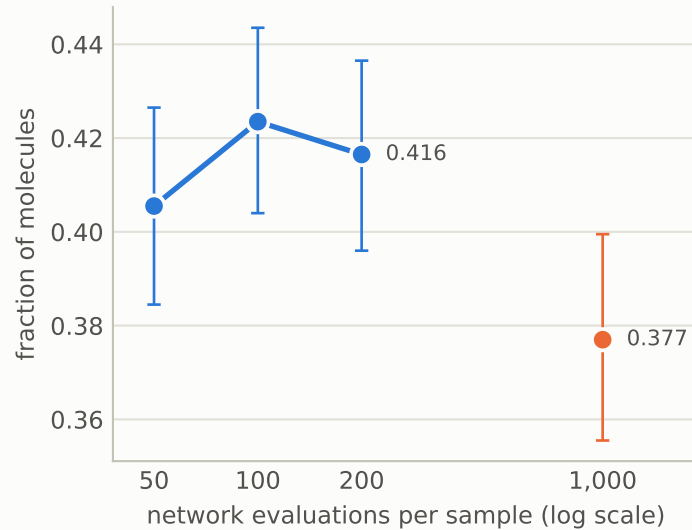
Validity
