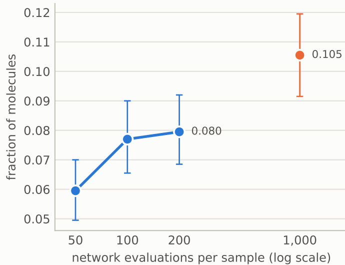
Molecule stability
