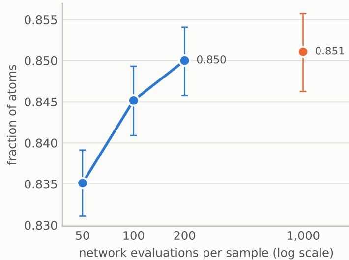
Atom stability
