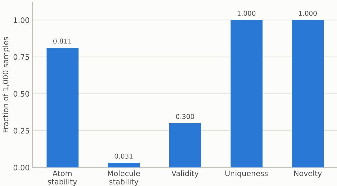
Sample quality, EGNN denoiser on QM9
