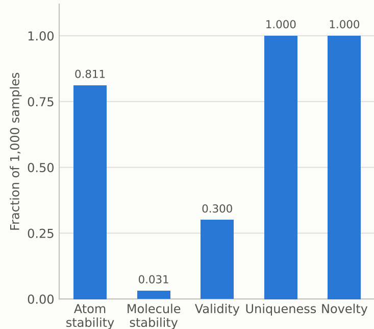
Sample quality, EGNN denoiser on QM9
