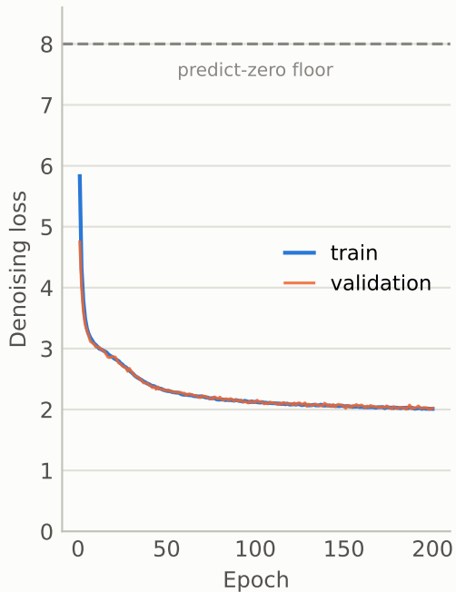
Training converged
