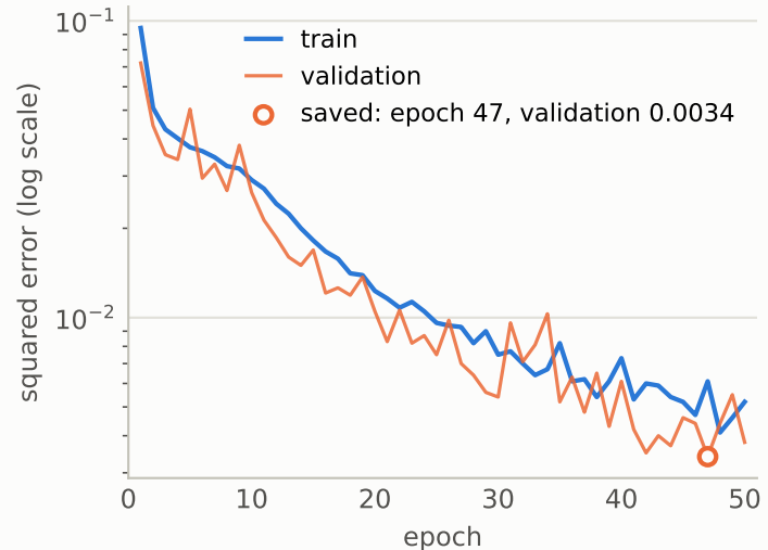
Property evaluator
