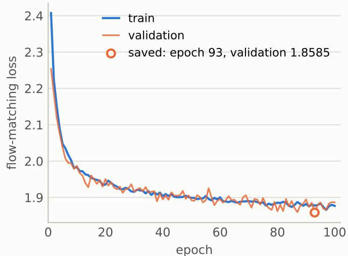
Flow matching
