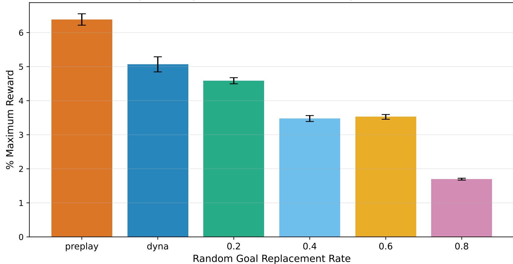
Dyna Multigoal: % Maximum Reward by Condition
