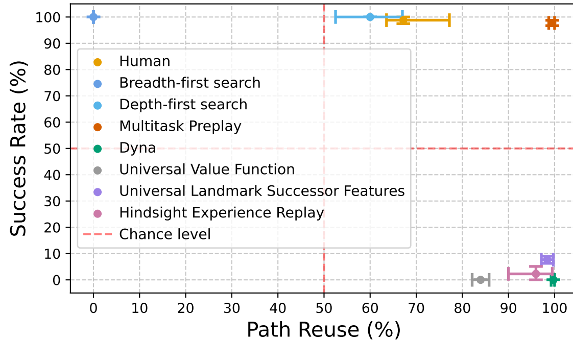
Threshold = 0.5
