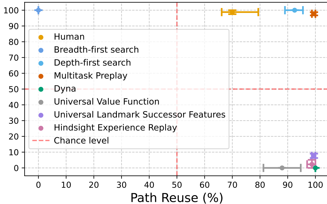
Threshold = 0.3
