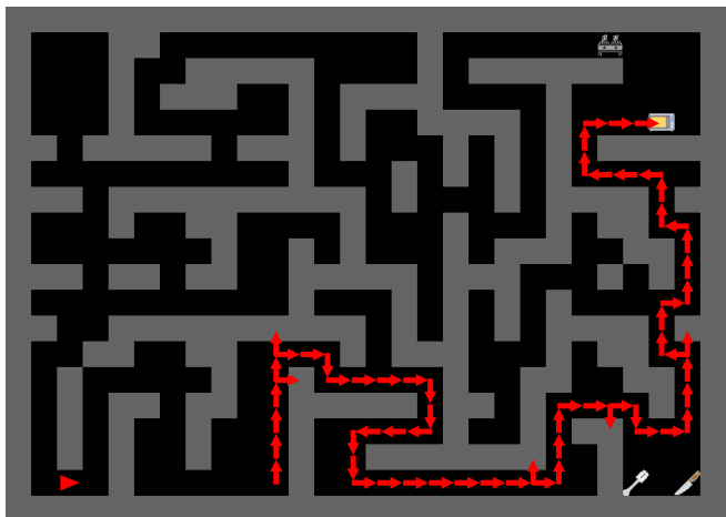
Train 2 (✓) | start_pos=[ 7 21]
