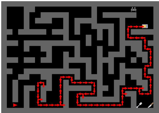
Train 6 (✓) | start_pos=[13 6]
