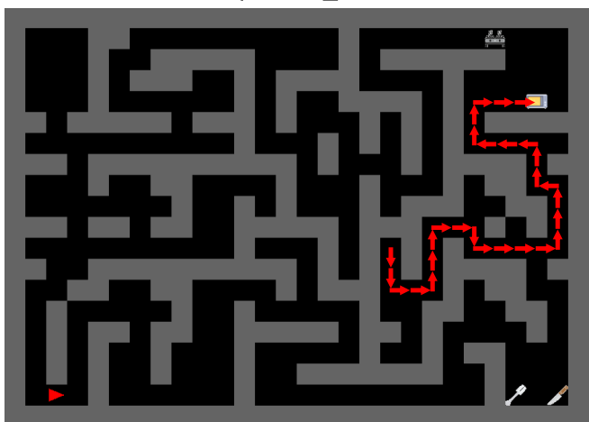
Train 4 (✓) | start_pos=[15 24]
