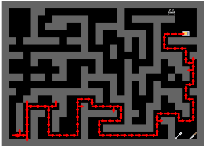
Train 7 (✓) | start_pos=[ 5 25]
