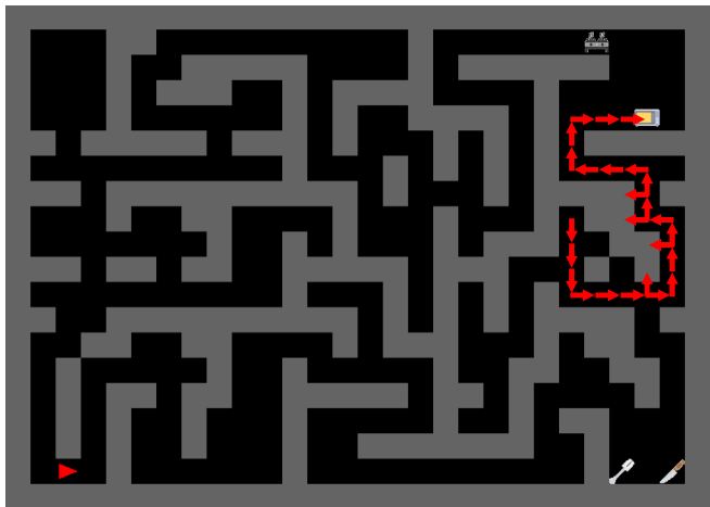
Train 3 (✓) | start_pos=[10 17]
