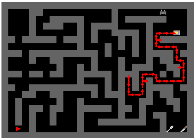
Train 1 (✓) | start_pos=[17 9]
