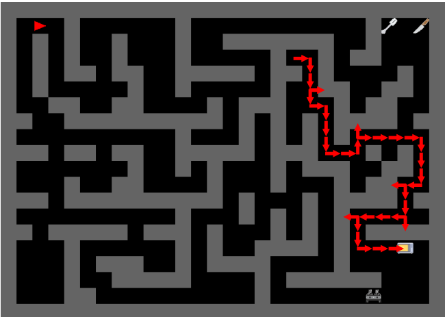
Train 1 (✓) | start pos=[10 21]
