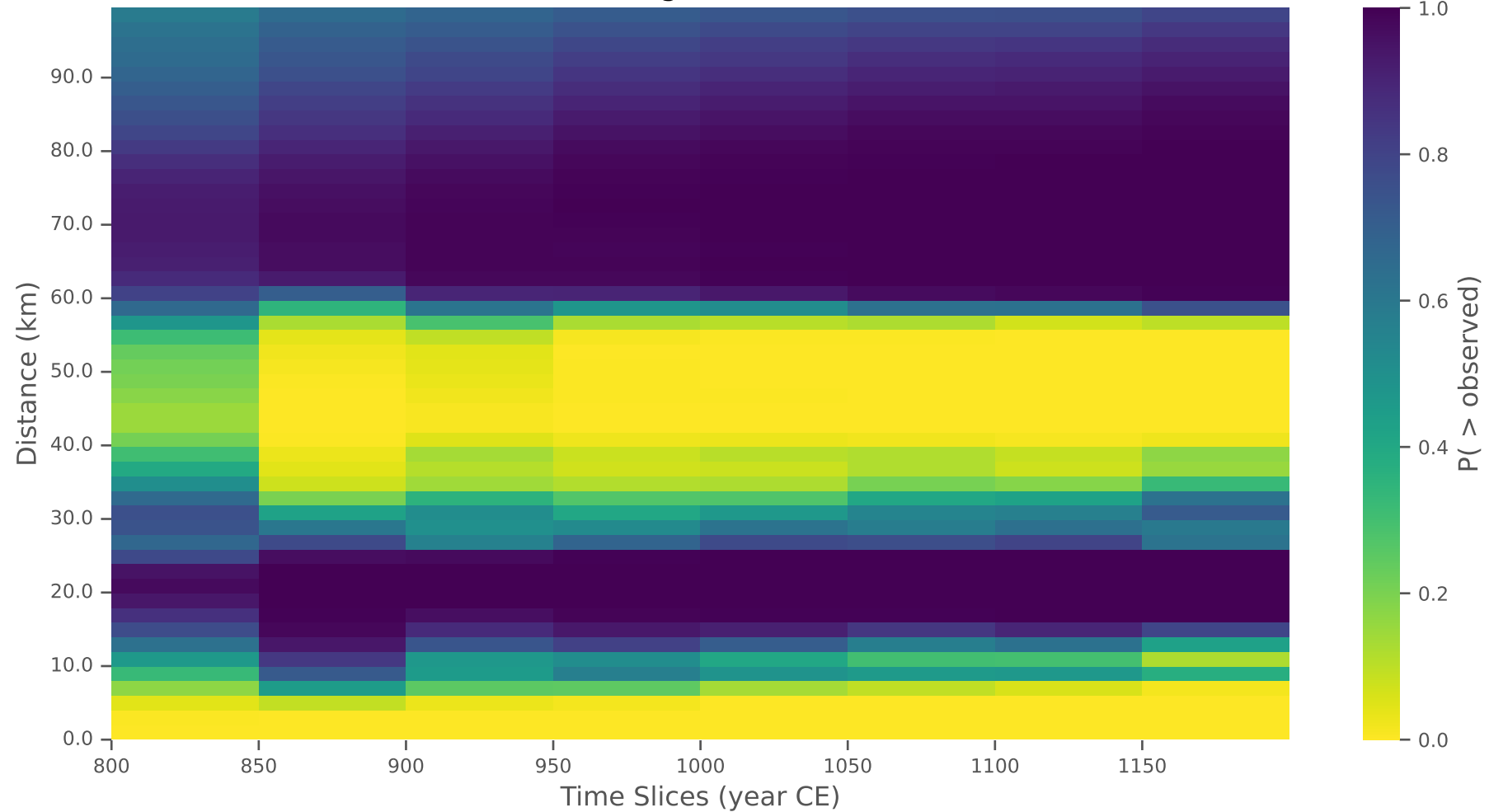
P-Values for Angkor PDD (BISE null)
