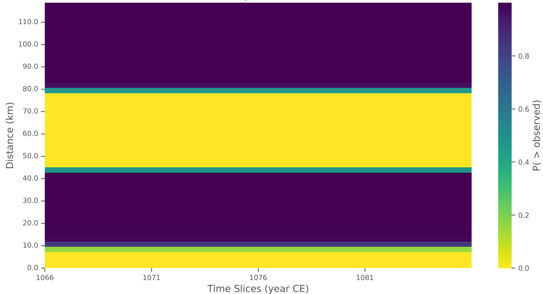
P-Values for Hamphsire PDD (BISE null)
