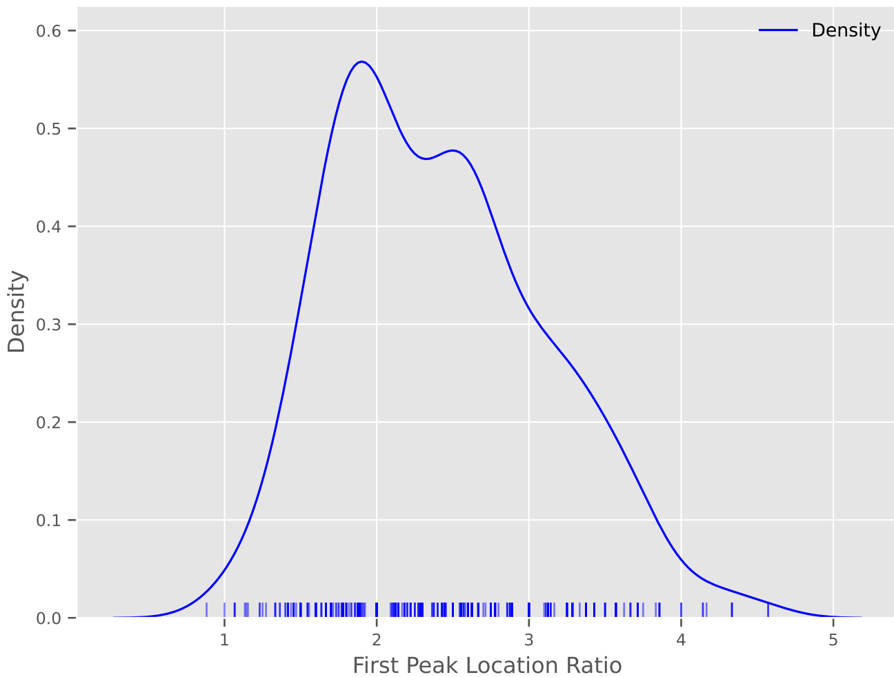
Distribution of First Peak Location Ratios
