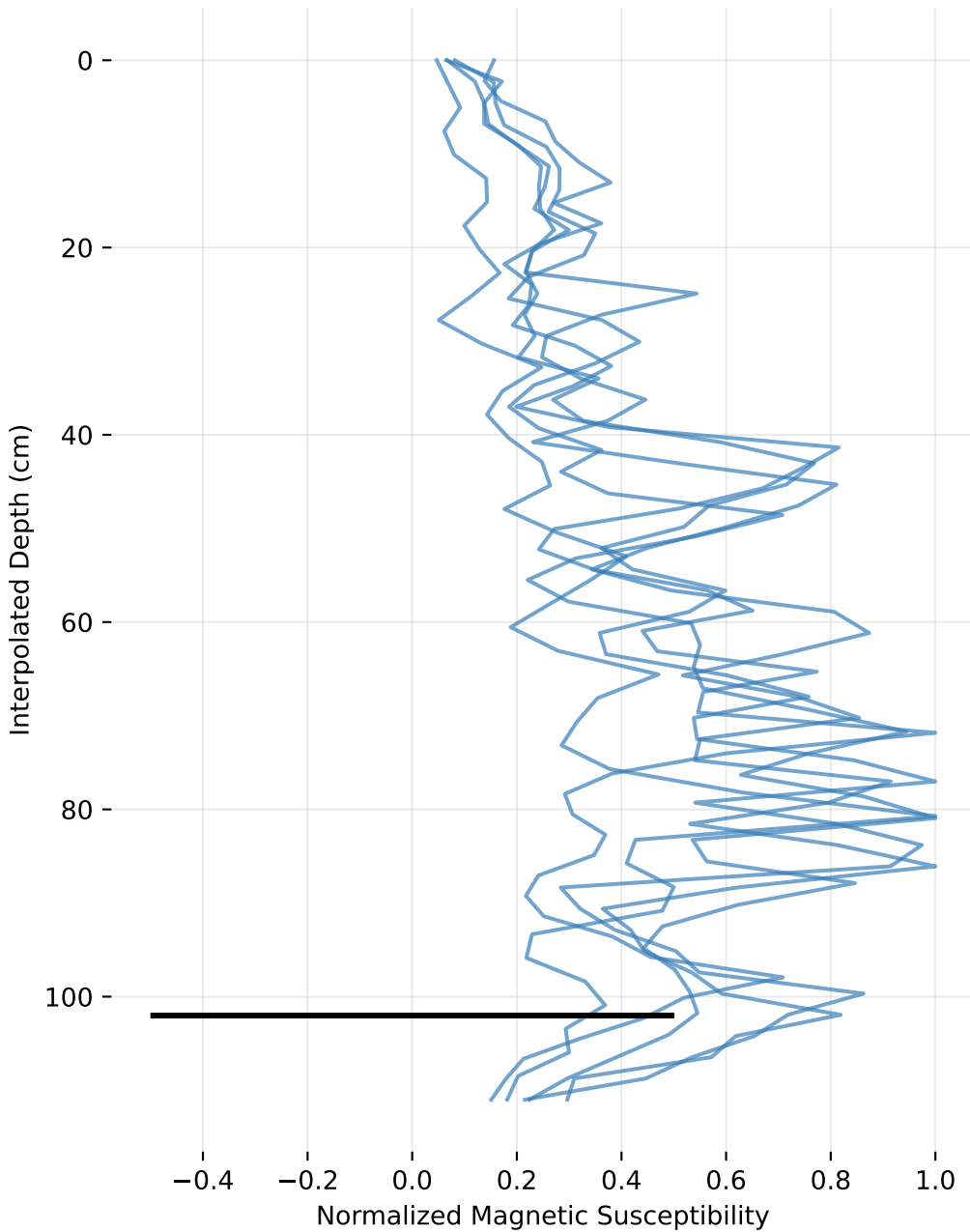
Magnetic Susceptibility Profile - Trench 7
