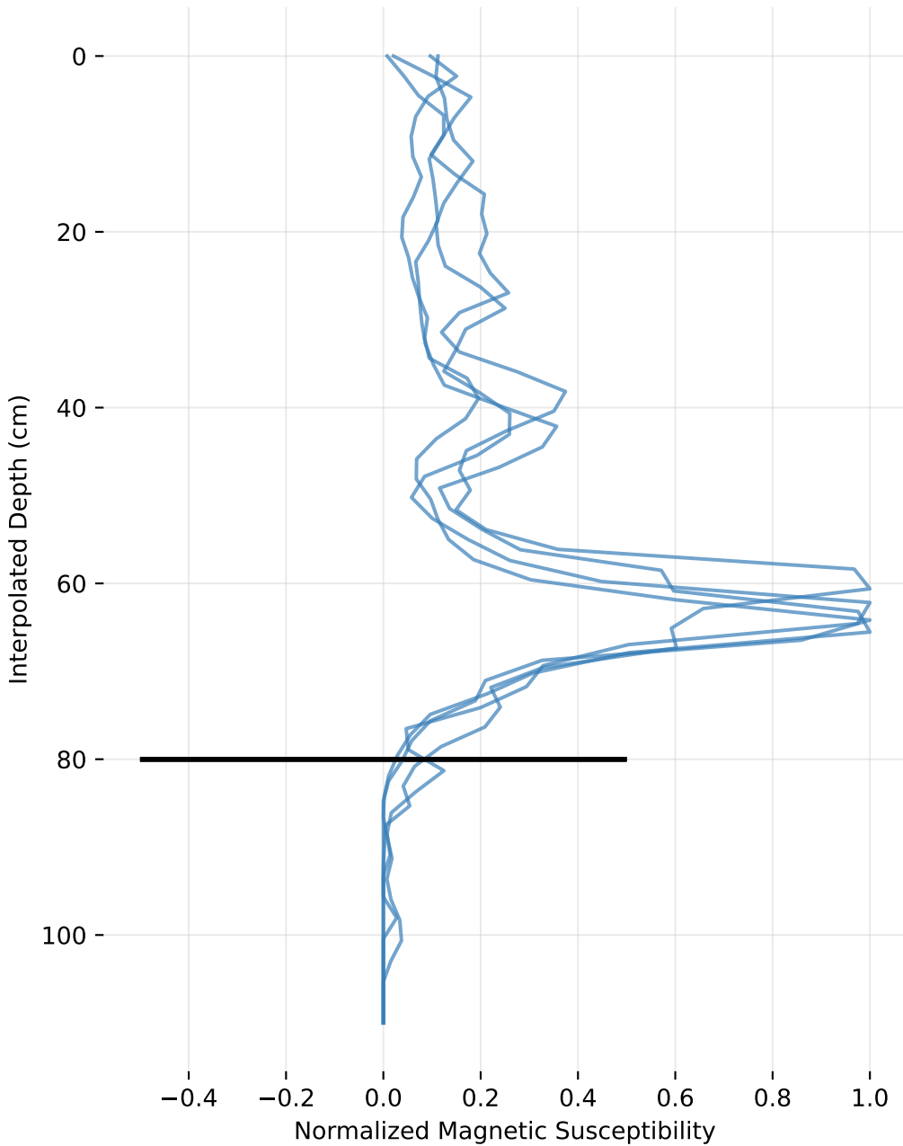
Magnetic Susceptibility Profile - Trench 3
