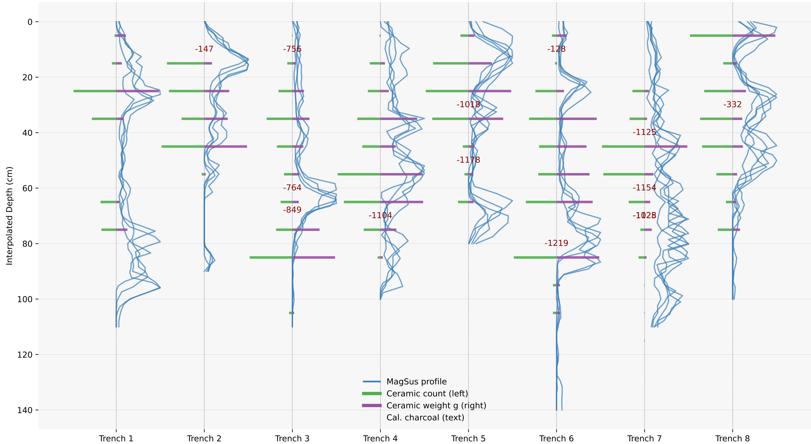
Magnetic Susceptibility Profiles with Ceramic Counts (left) & Weights (right)
