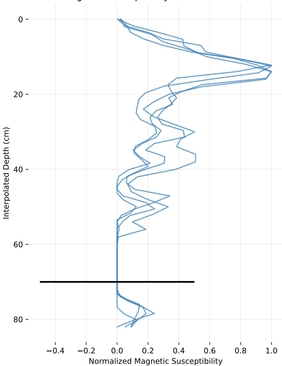
Magnetic Susceptibility Profile - Trench 2
