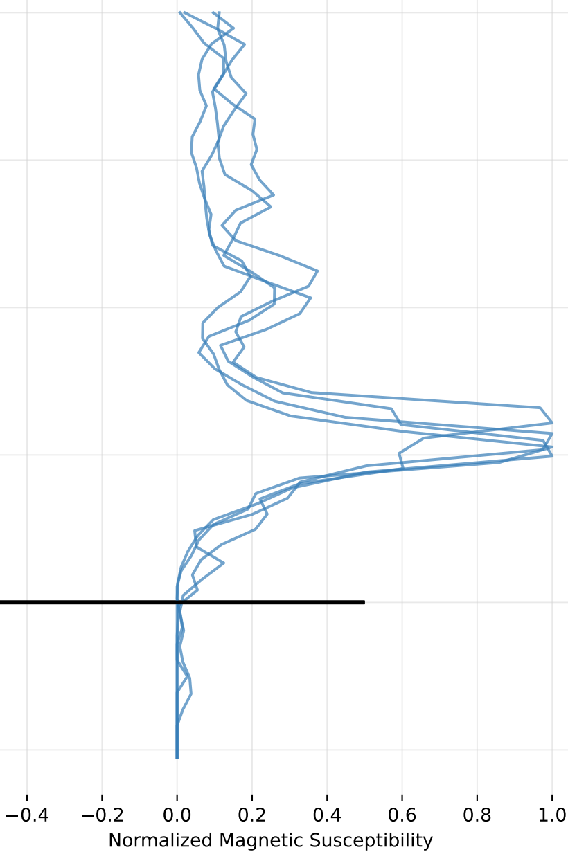
Magnetic Susceptibility Profile - Trench 3
