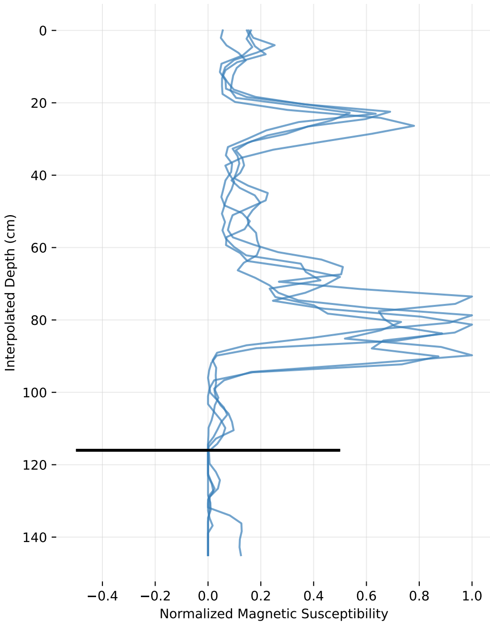
Magnetic Susceptibility Profile - Trench 6
