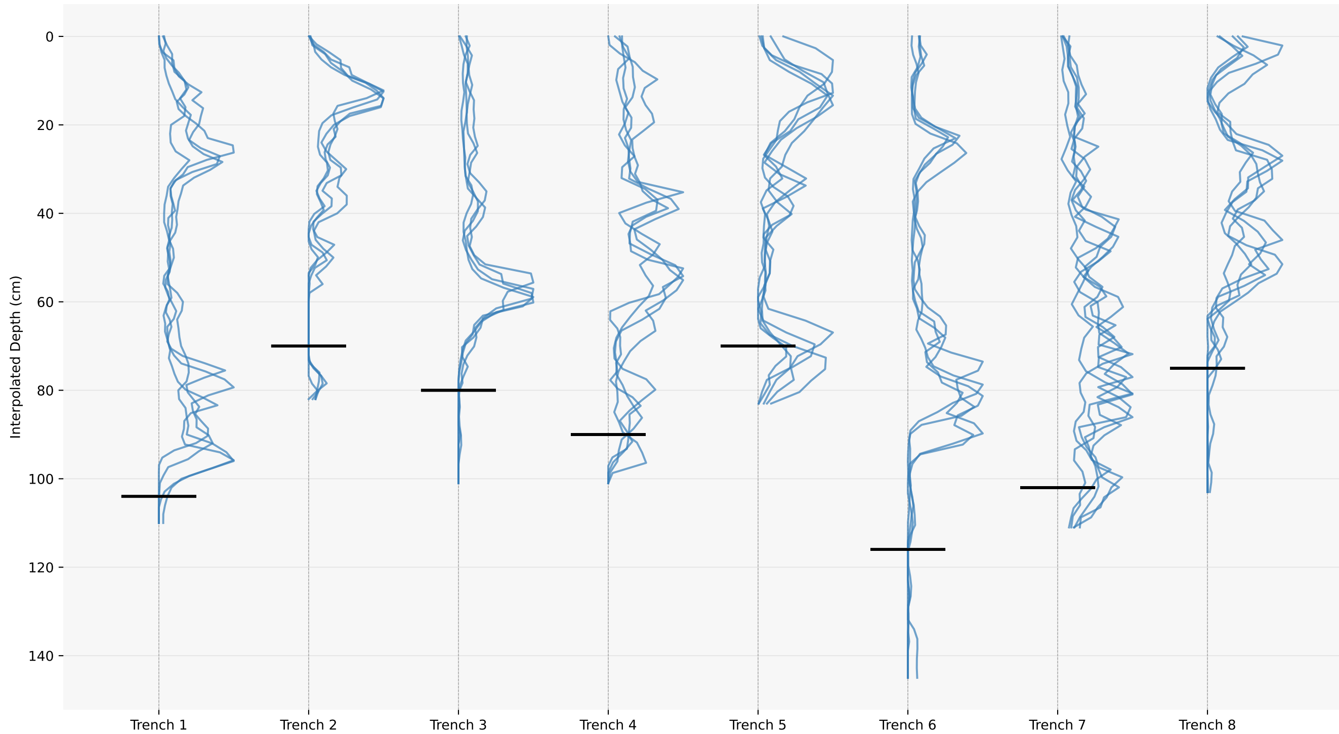
Magnetic Susceptibility Profiles (All Trenches)
