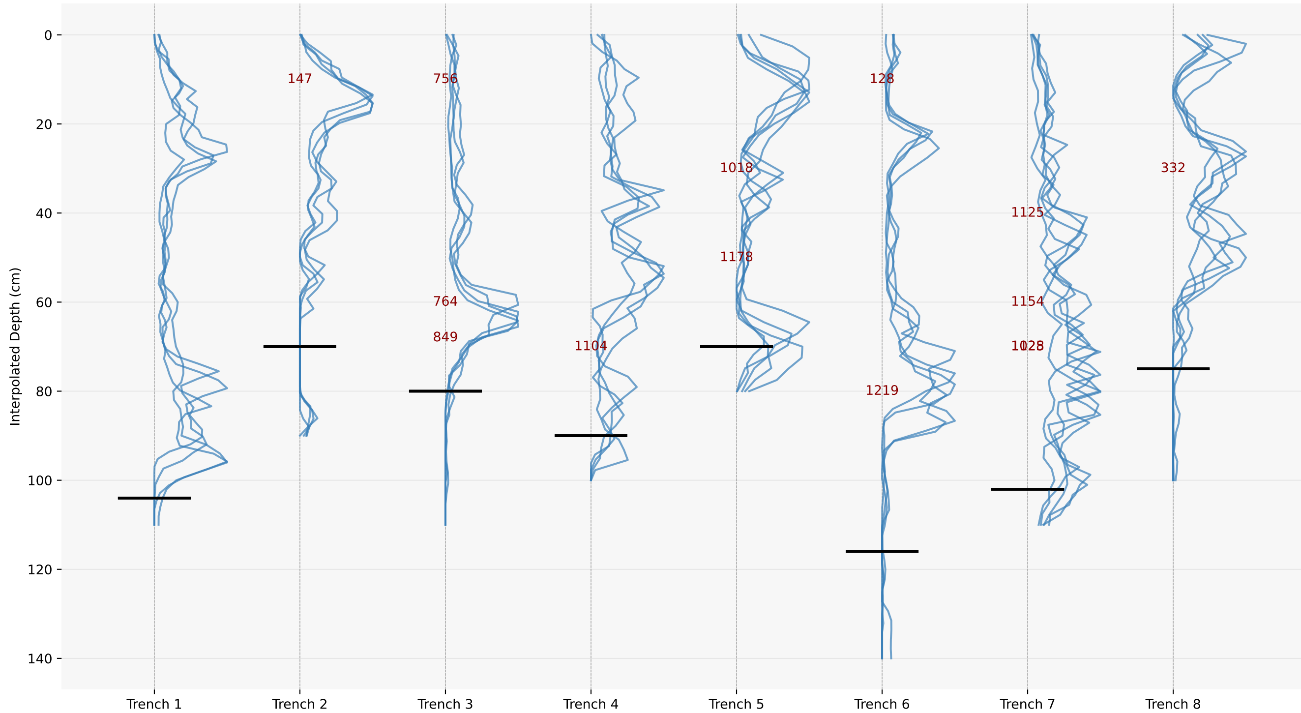
Magnetic Susceptibility Profiles (All Trenches) with Calibrated Charcoal Dates
