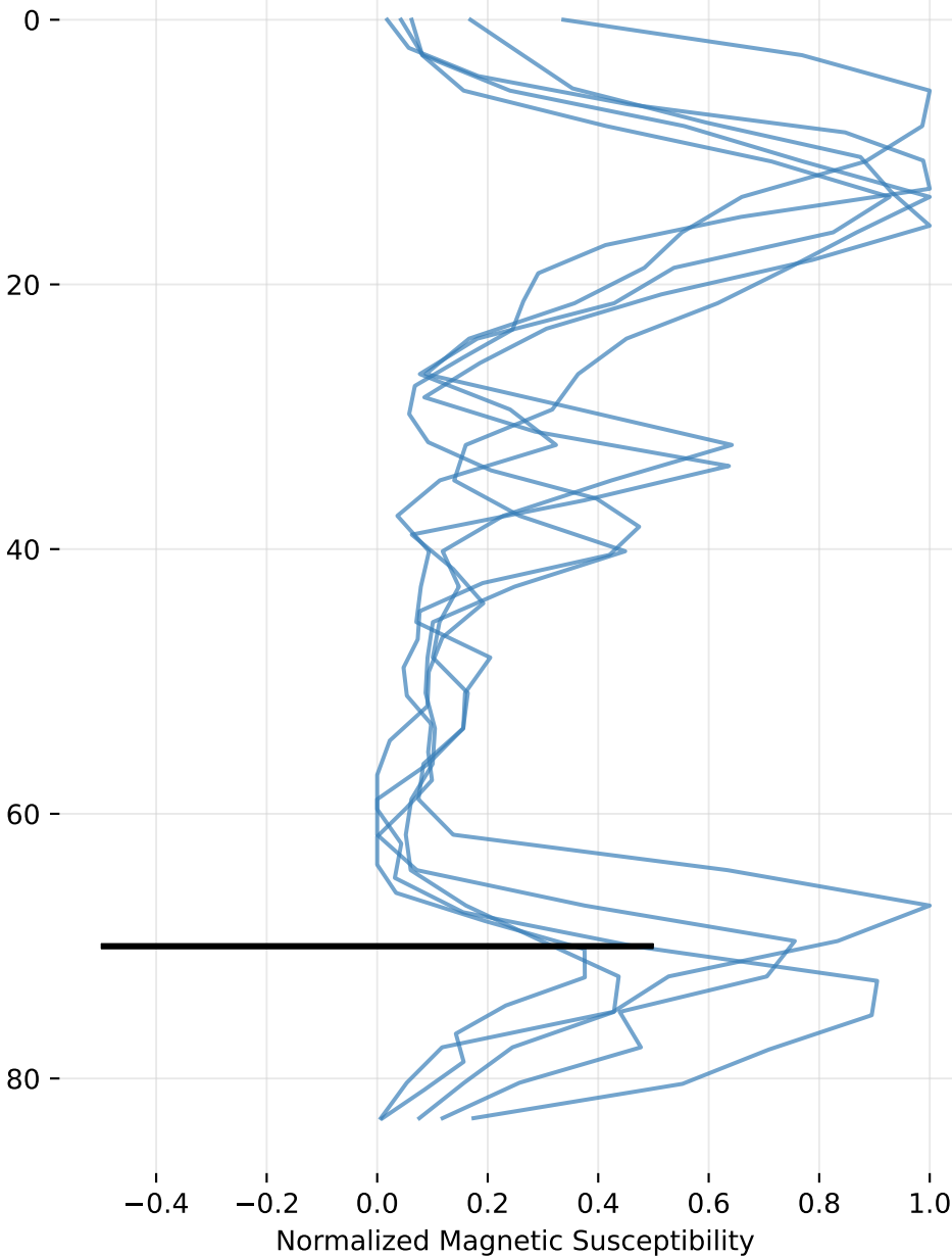
Magnetic Susceptibility Profile - Trench 5
