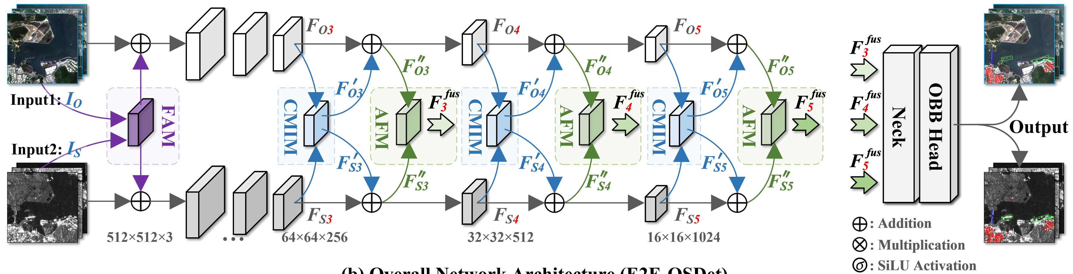
(b) Overall Network Architecture (E2E-OSDet)
