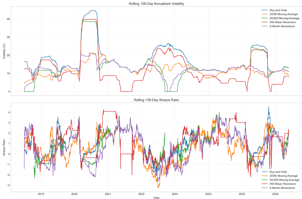
v7_rolling_risk.png
