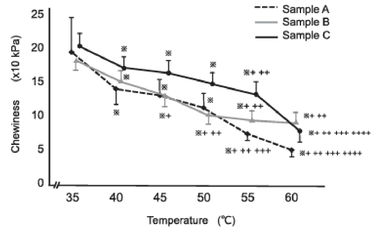
Fig. 12 Relationship between temperature and chewiness for each sample. All three samples showed an increase in chewiness with decreasing temperature (Mean \pm SD, * p < 0.05 vs 35°C, + p < 0.05 vs 40°C, ++ p < 0.05 vs 45°C, +++ p < 0.05 vs 50°C, ++++ p < 0.05 vs 55°C, n = 10).
