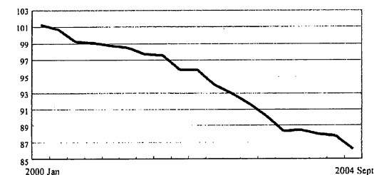
GDP Deflator
