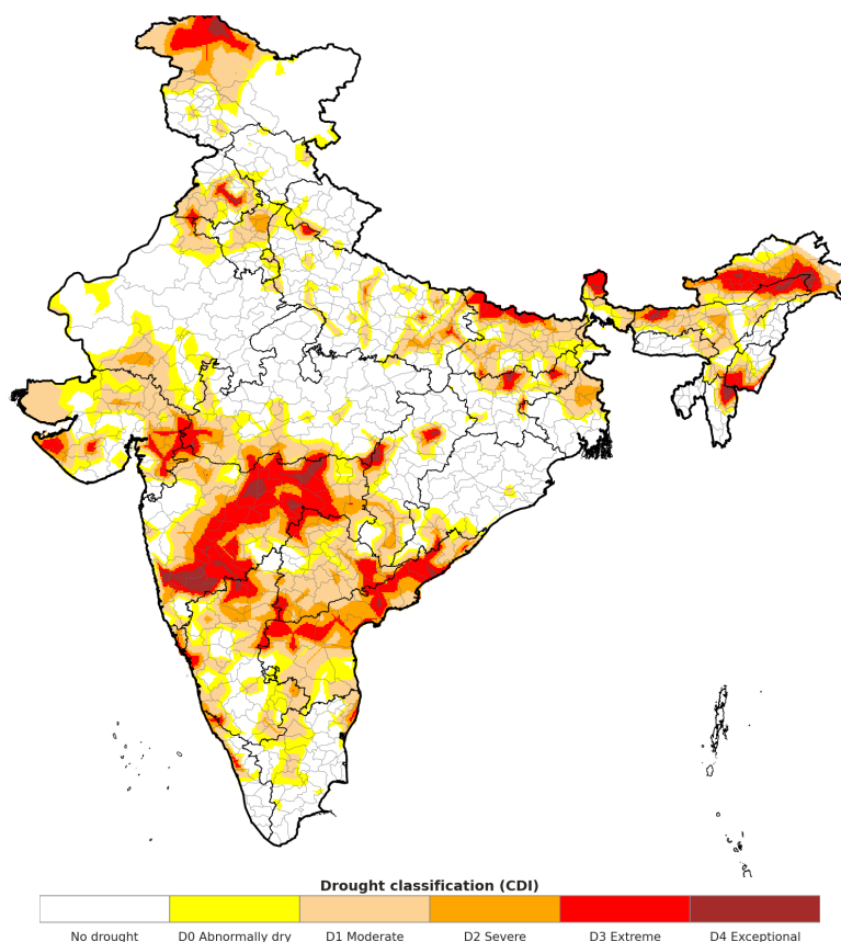
Combined Drought Index (CDI) for the week ending September 9, 2026.
