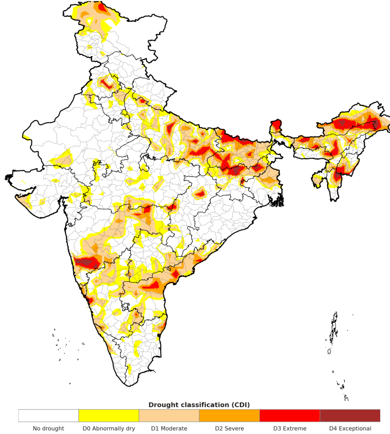
Combined Drought Index (CDI) for the week ending August 26, 2026.
