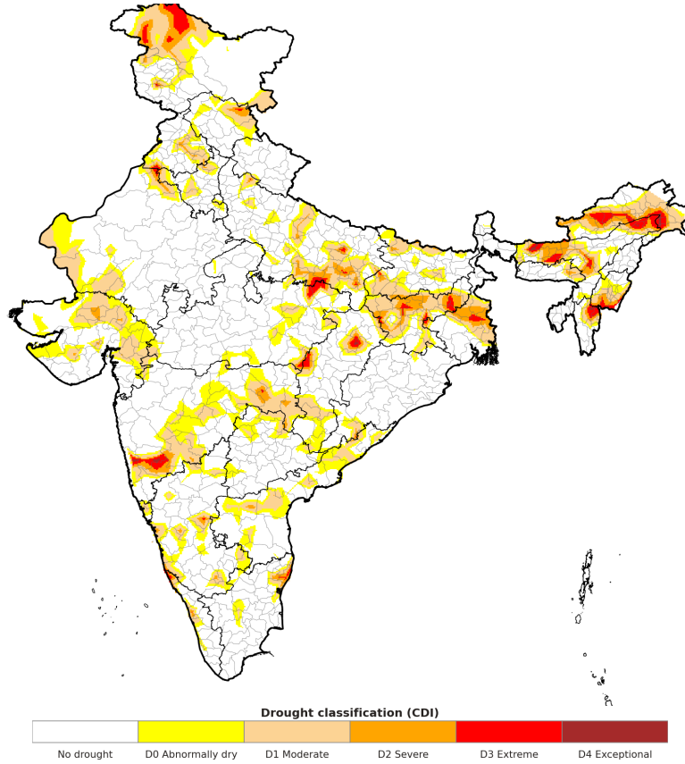
Combined Drought Index (CDI) for the week ending July 22, 2026.
