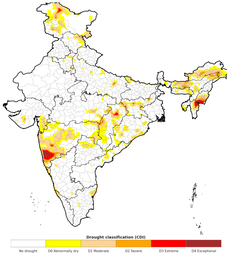
Combined Drought Index (CDI) for the week ending June 17, 2026.
