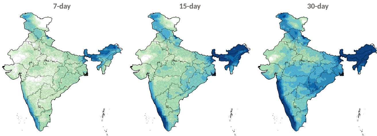
Forecast runoff for the 7-, 15- and 30-day horizons, initialized May 20, 2026.
