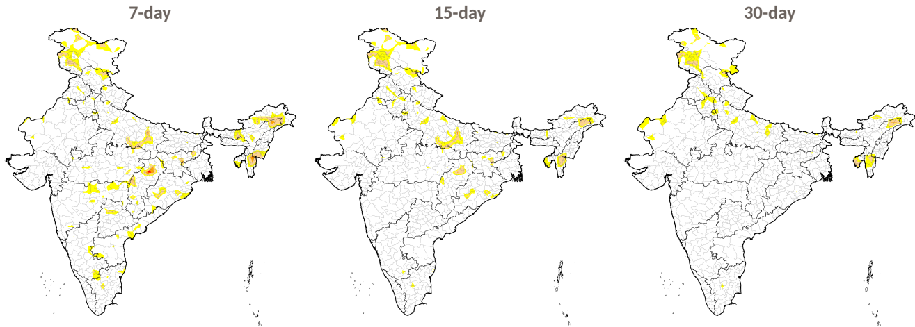
Forecast drought (cdi) for the 7-, 15- and 30-day horizons, initialized May 20, 2026.
